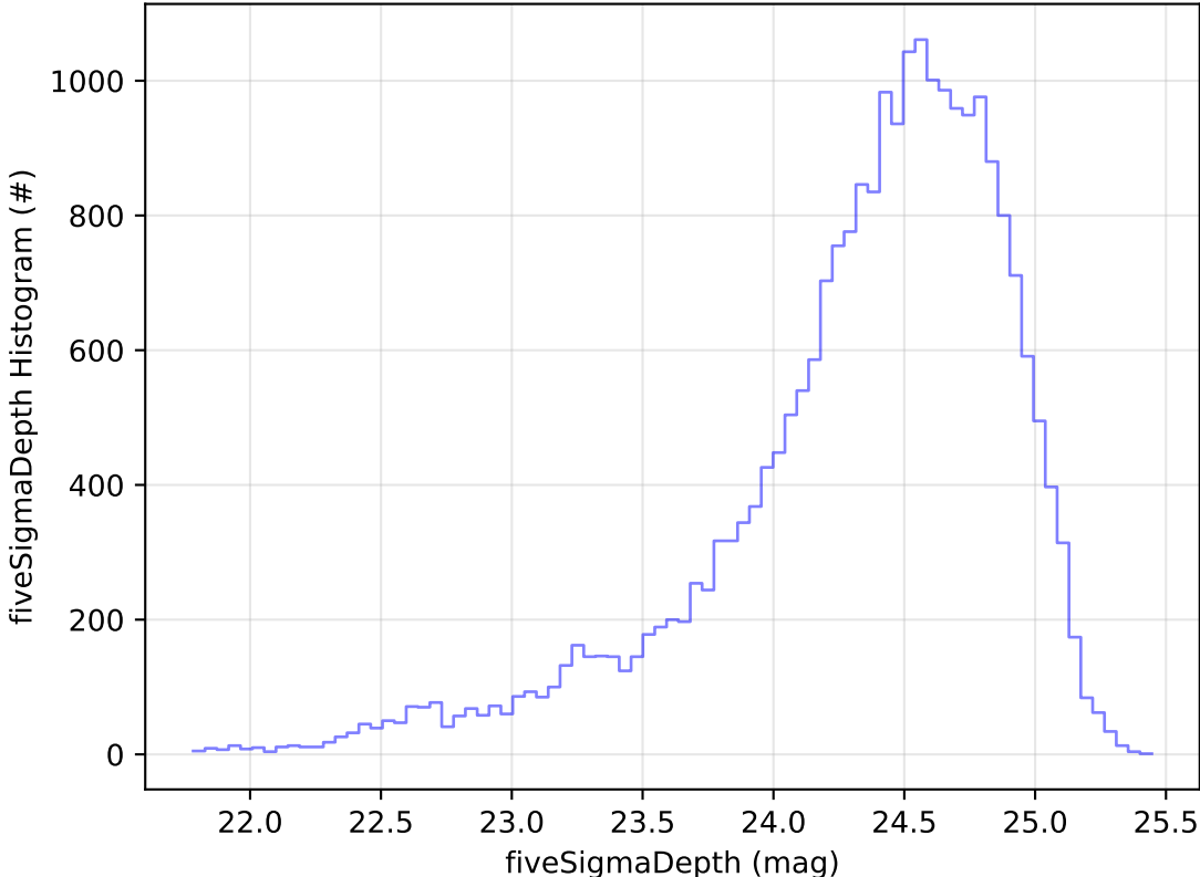
too_elab_r128_d2_griz_v3.4_10yrs Yr 1 g band: fiveSigmaDepth Histogram
