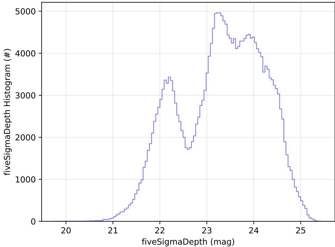
too_elab_r128_d2_griz_v3.4_10yrs Yr 1 all bands: fiveSigmaDepth Histogram
