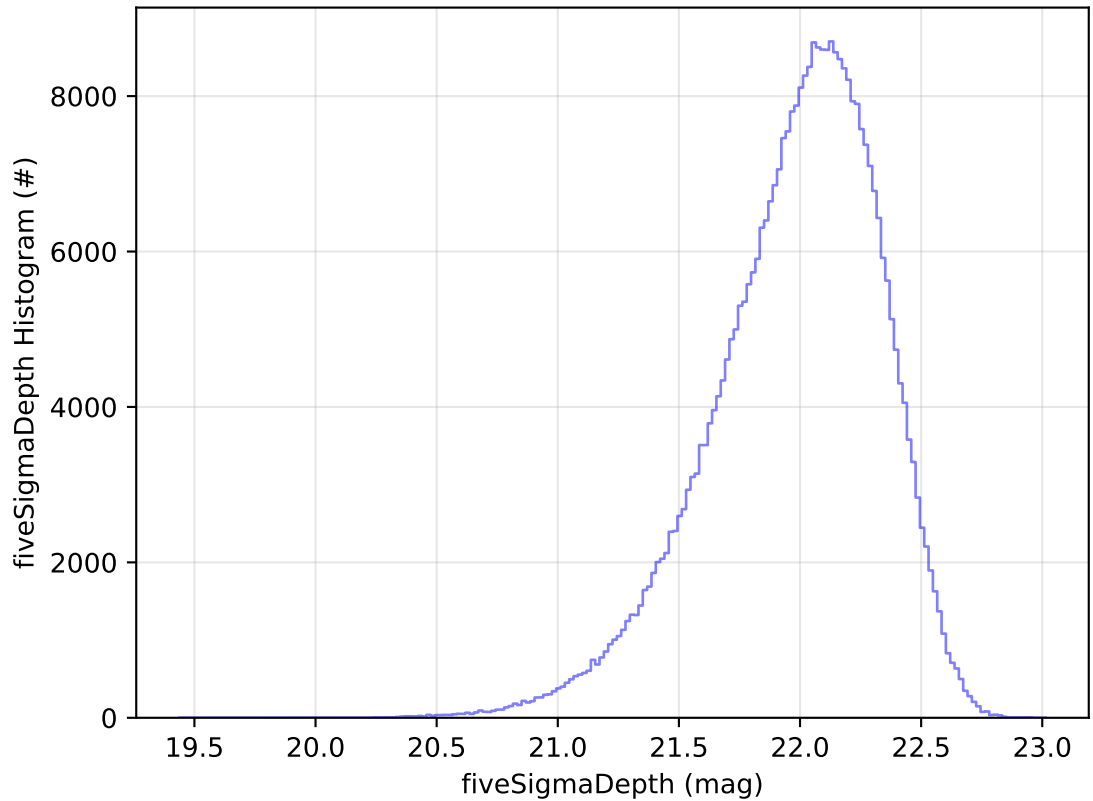
too_elab_r128_d2_griz_v3.4_10yrs WFD y band: fiveSigmaDepth Histogram
