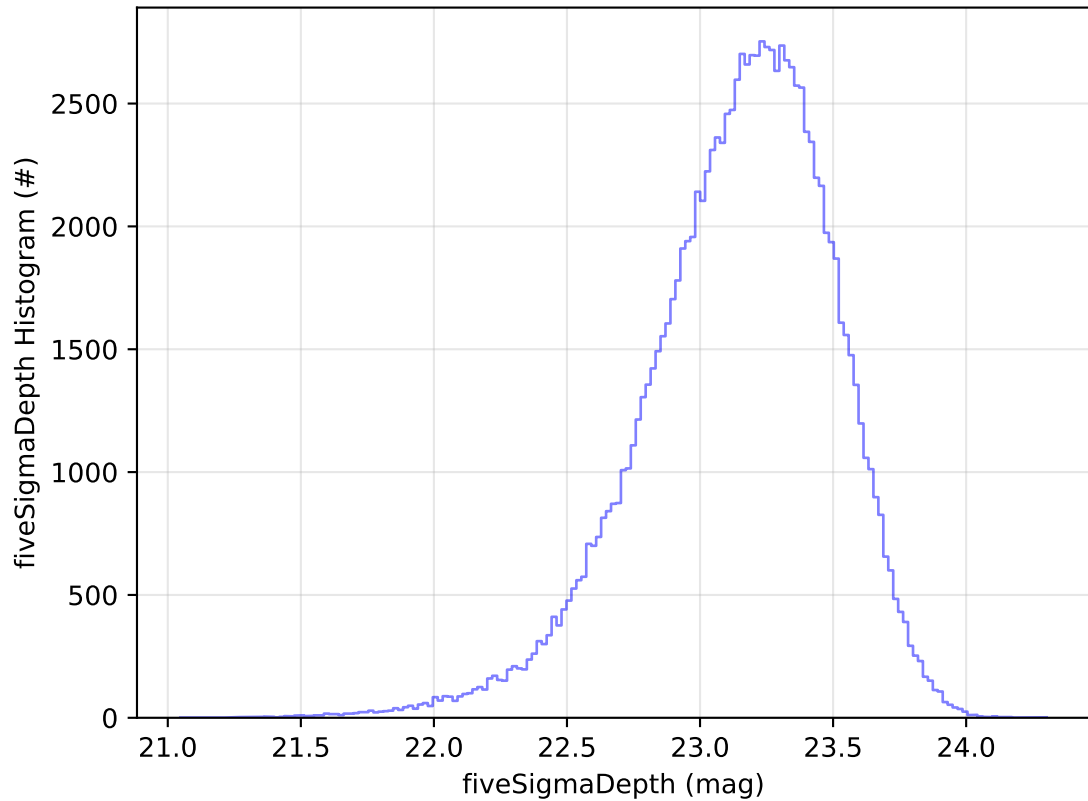
too_elab_r128_d2_griz_v3.4_10yrs WFD u band: fiveSigmaDepth Histogram
