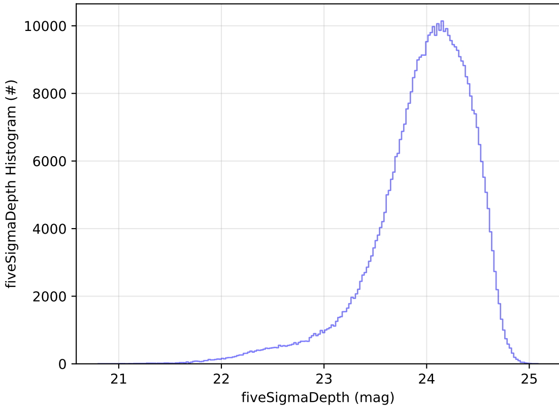
too_elab_r128_d2_griz_v3.4_10yrs WFD r band: fiveSigmaDepth Histogram
