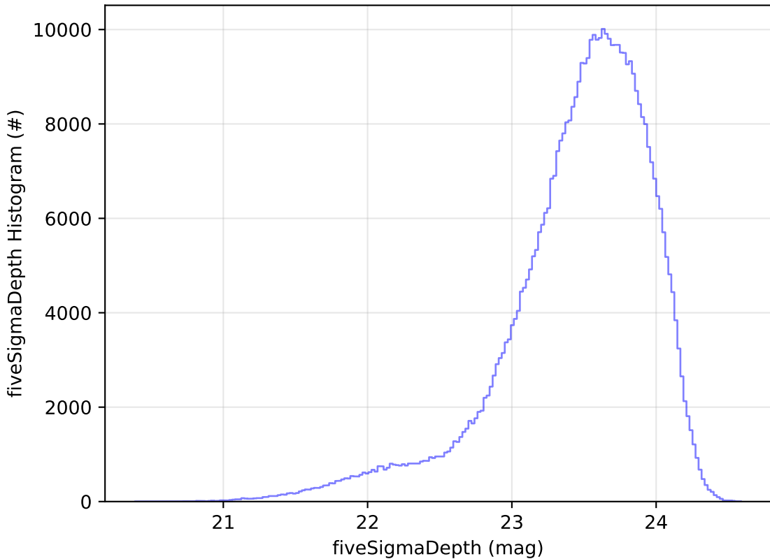
too_elab_r128_d2_griz_v3.4_10yrs WFD i band: fiveSigmaDepth Histogram
