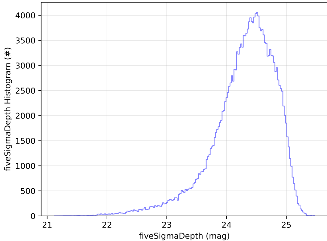
too_elab_r128_d2_griz_v3.4_10yrs WFD g band: fiveSigmaDepth Histogram
