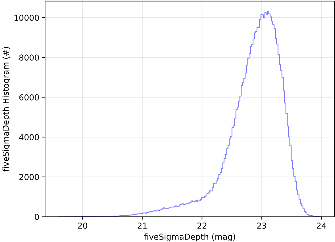
too_elab_r128_d2_griz_v3.4_10yrs All sky z band: fiveSigmaDepth Histogram
