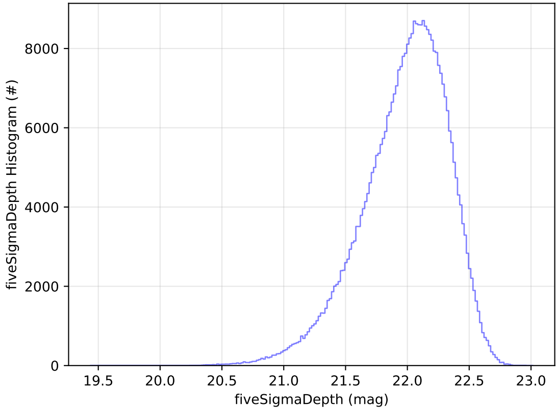
too_elab_r128_d2_griz_v3.4_10yrs All sky y band: fiveSigmaDepth Histogram
