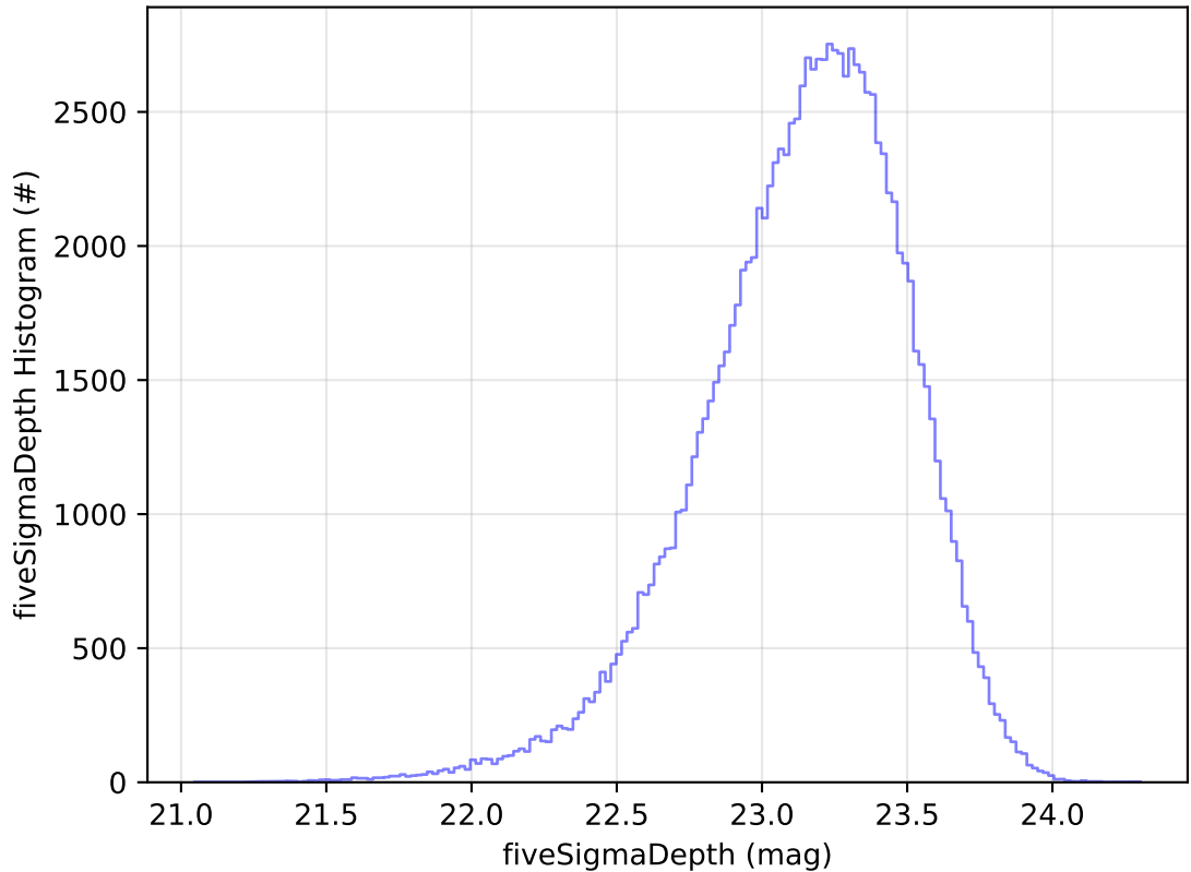
too_elab_r128_d2_griz_v3.4_10yrs All sky u band: fiveSigmaDepth Histogram
