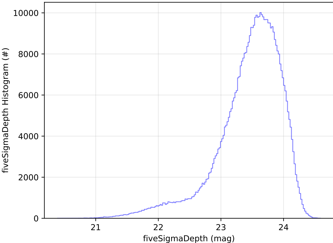
too_elab_r128_d2_griz_v3.4_10yrs All sky i band: fiveSigmaDepth Histogram
