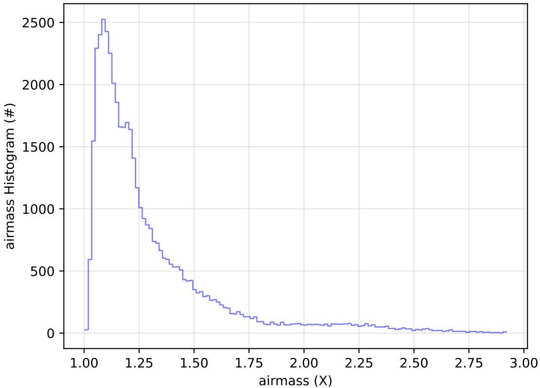
too_elab_r128_d2_griz_v3.4_10yrs Yr 1 z band: airmass Histogram
