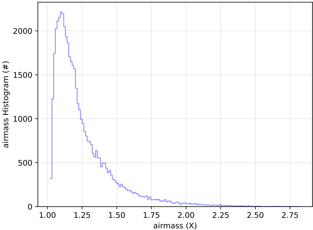
too_elab_r128_d2_griz_v3.4_10yrs Yr 1 y band: airmass Histogram
