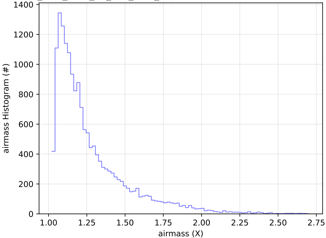
too_elab_r128_d2_griz_v3.4_10yrs Yr 1 u band: airmass Histogram
