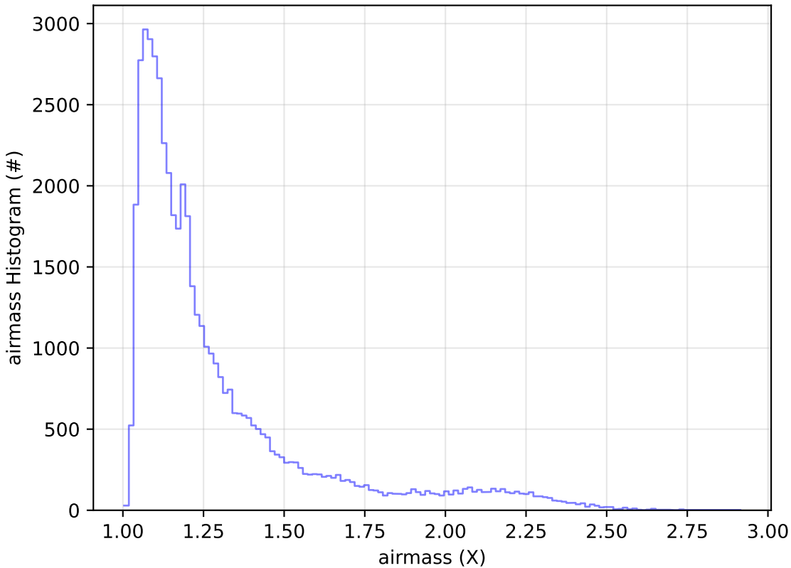
too_elab_r128_d2_griz_v3.4_10yrs Yr 1 r band: airmass Histogram
