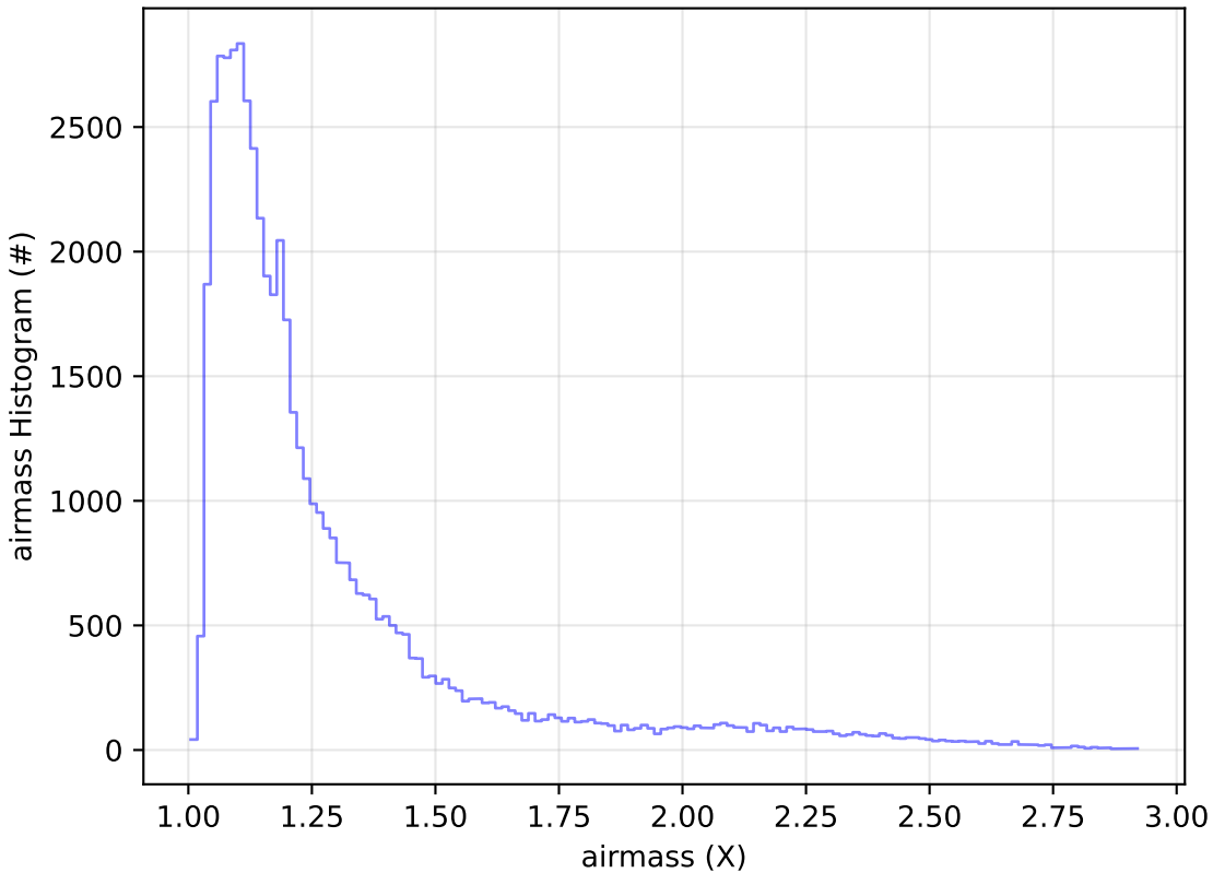
too_elab_r128_d2_griz_v3.4_10yrs Yr 1 i band: airmass Histogram
