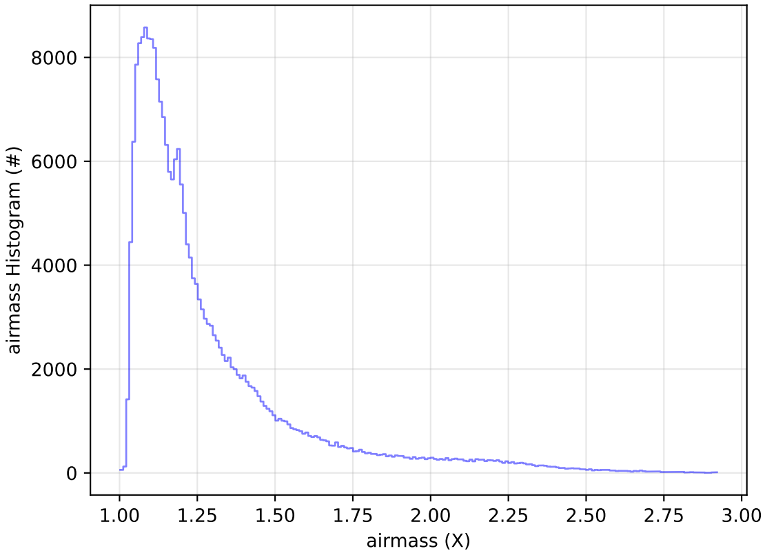
too_elab_r128_d2_griz_v3.4_10yrs Yr 1 all bands: airmass Histogram
