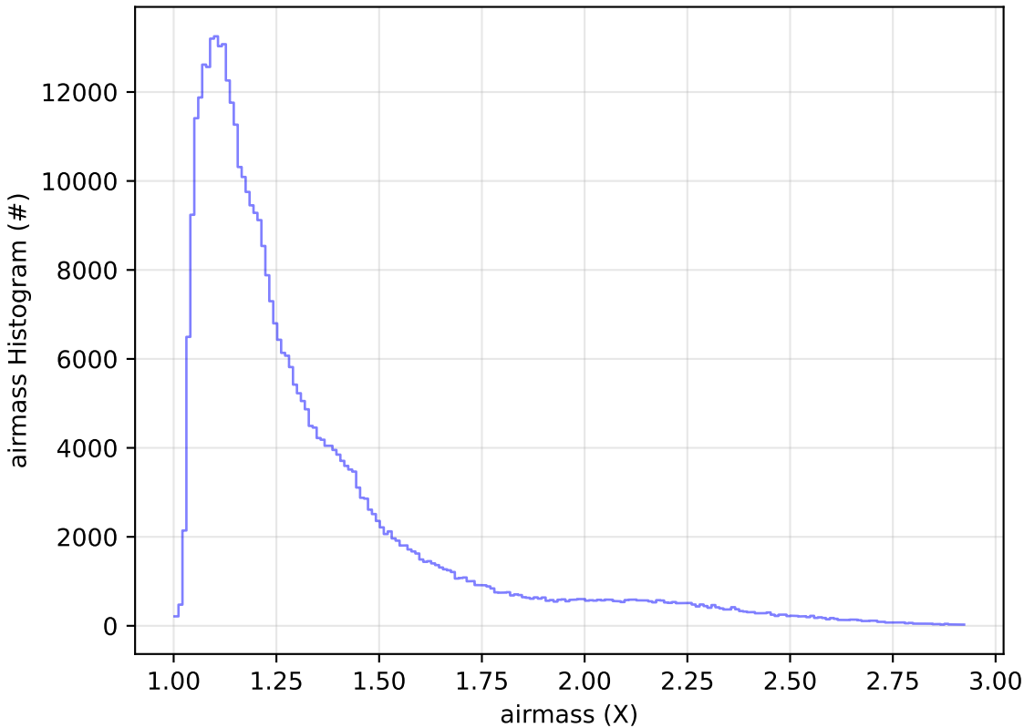
too_elab_r128_d2_griz_v3.4_10yrs WFD z band: airmass Histogram
