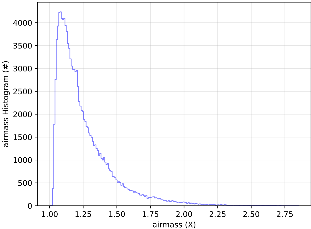
too_elab_r128_d2_griz_v3.4_10yrs WFD u band: airmass Histogram
