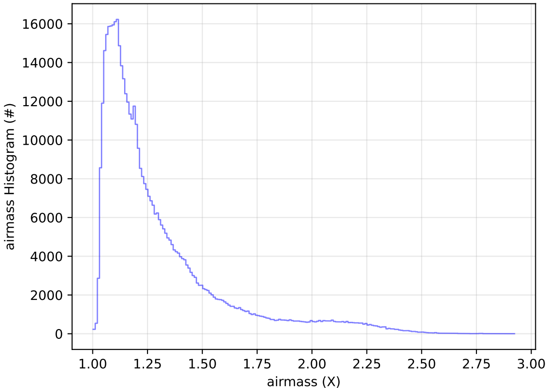
too_elab_r128_d2_griz_v3.4_10yrs WFD r band: airmass Histogram
