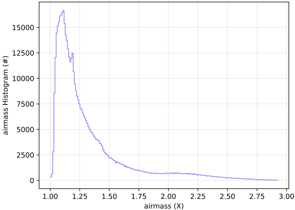
too_elab_r128_d2_griz_v3.4_10yrs WFD i band: airmass Histogram
