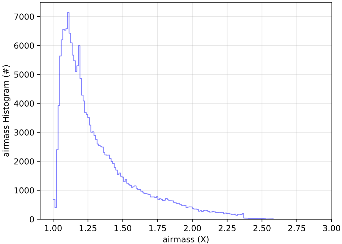
too_elab_r128_d2_griz_v3.4_10yrs WFD g band: airmass Histogram
