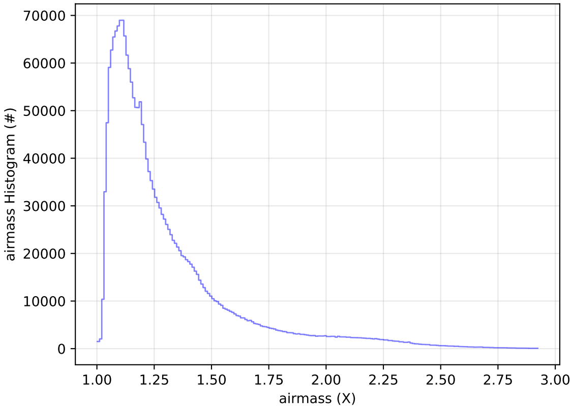
too_elab_r128_d2_griz_v3.4_10yrs WFD all bands: airmass Histogram
