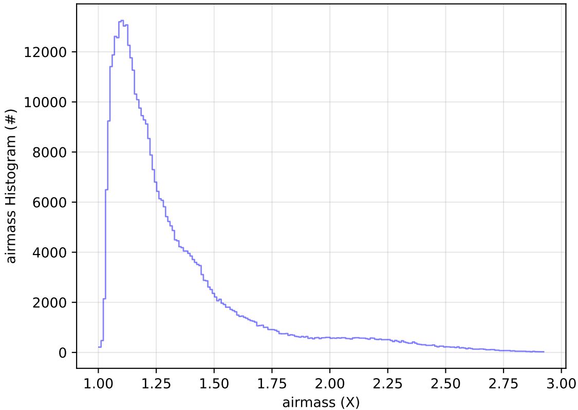
too_elab_r128_d2_griz_v3.4_10yrs All sky z band: airmass Histogram
