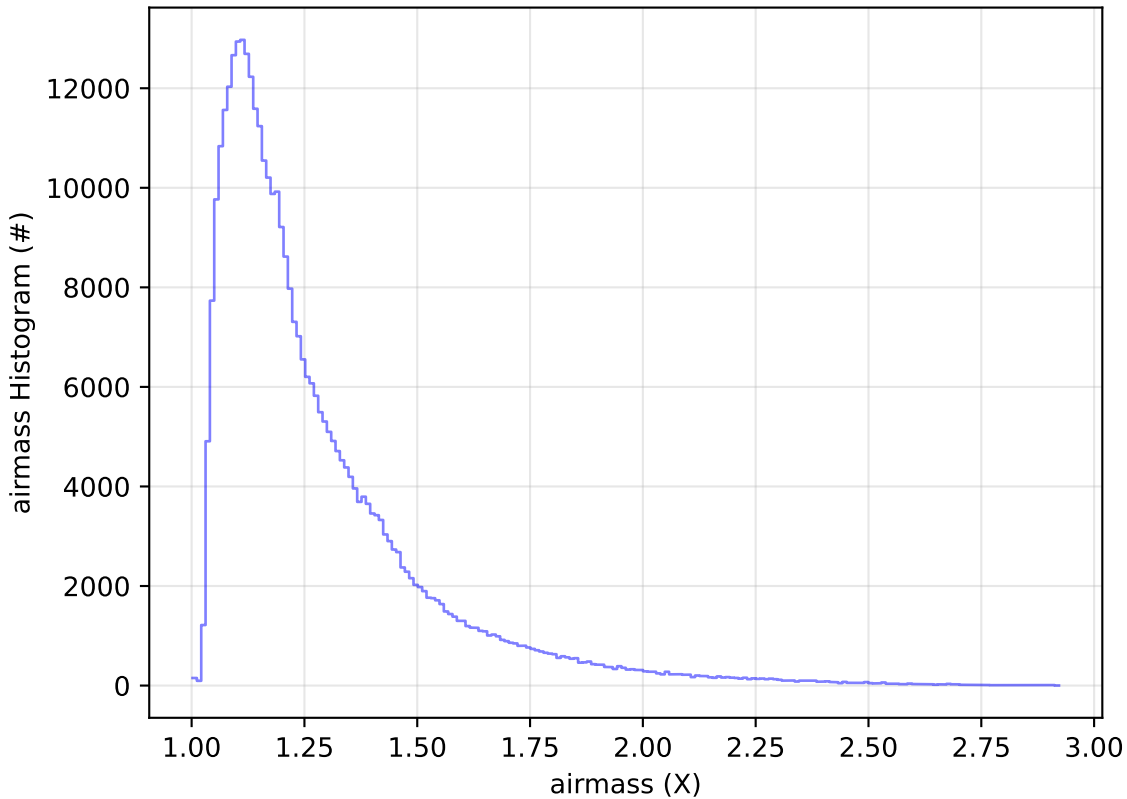
too_elab_r128_d2_griz_v3.4_10yrs All sky y band: airmass Histogram
