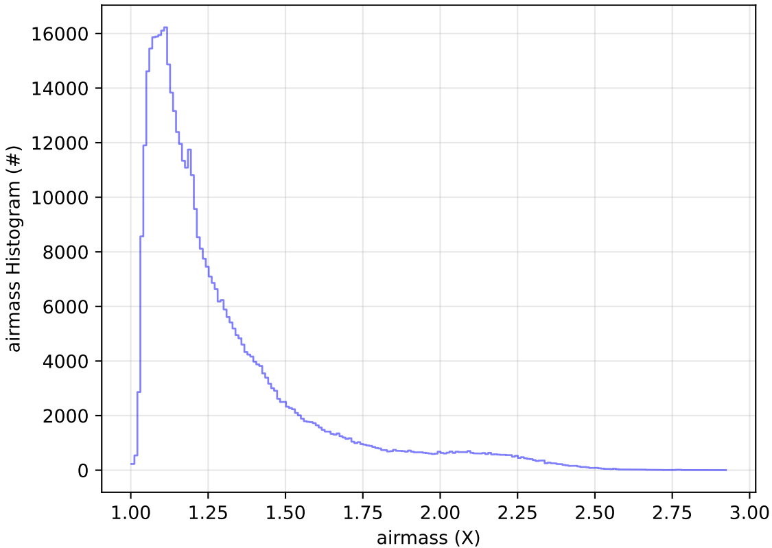
too_elab_r128_d2_griz_v3.4_10yrs All sky r band: airmass Histogram
