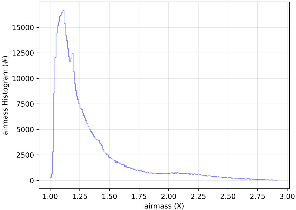
too_elab_r128_d2_griz_v3.4_10yrs All sky i band: airmass Histogram
