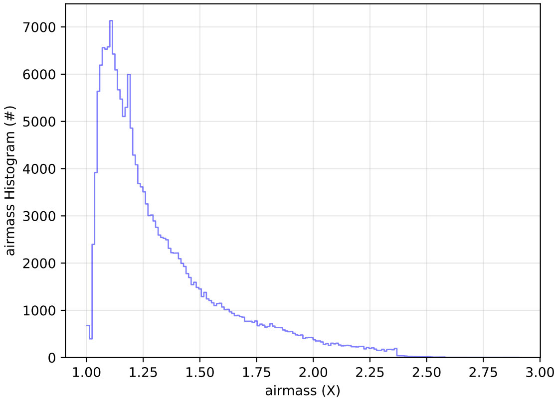
too_elab_r128_d2_griz_v3.4_10yrs All sky g band: airmass Histogram
