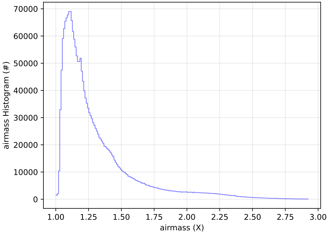
too_elab_r128_d2_griz_v3.4_10yrs All sky all bands: airmass Histogram
