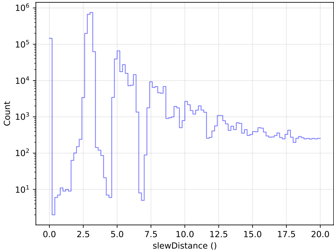
too_elab_r128_d2_griz_v3.4_10yrs All visits: Zoom Slew Distance Histogram
