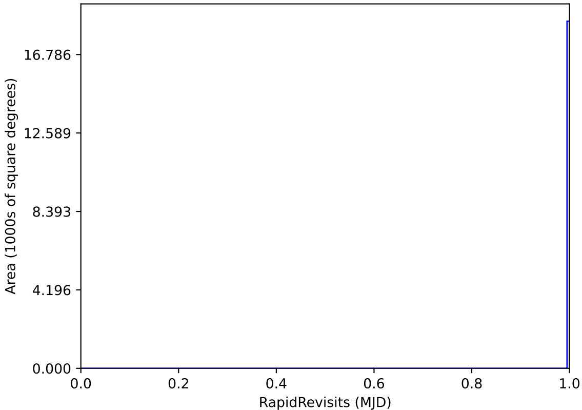
too_elab_r128_d2_griz_v3.4_10yrs WFD: RapidRevisits
