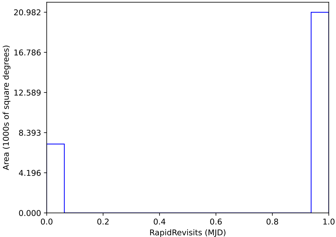
too_elab_r128_d2_griz_v3.4_10yrs All sky: RapidRevisits
