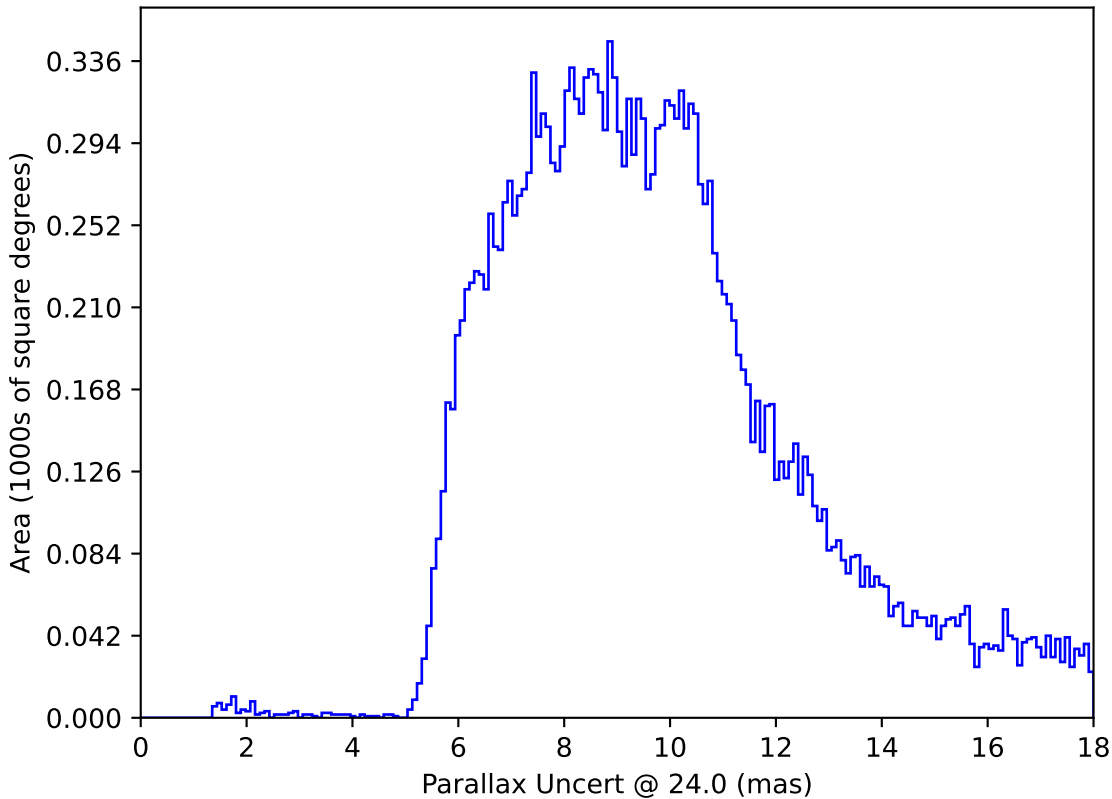
too_elab_r128_d2_griz_v3.4_10yrs All sky: Parallax Uncert @ 24.0
