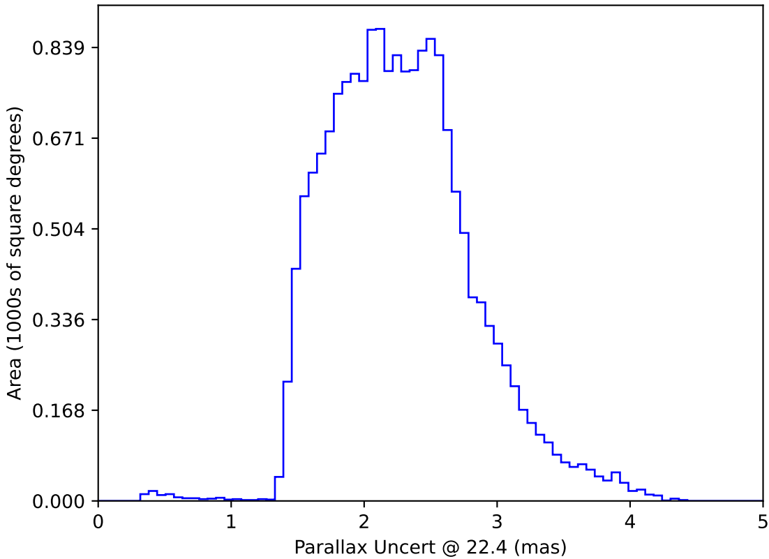
too_elab_r128_d2_griz_v3.4_10yrs WFD: Parallax Uncert @ 22.4
