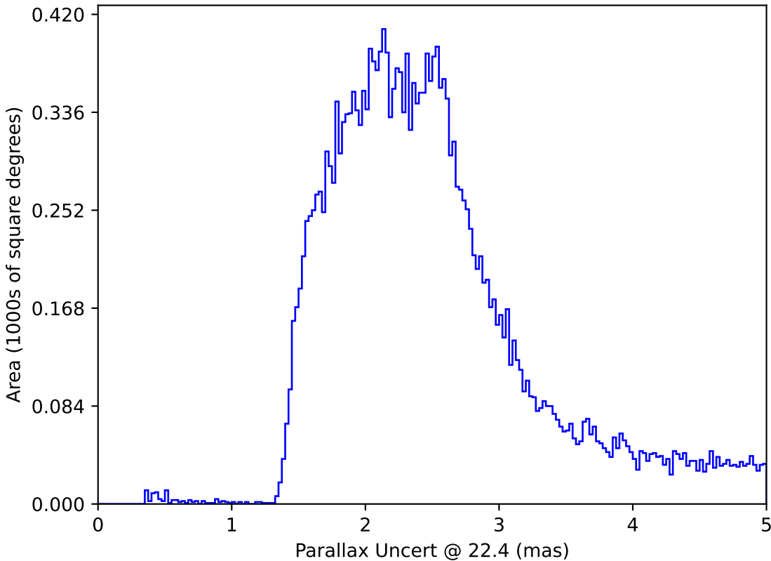
too_elab_r128_d2_griz_v3.4_10yrs All sky: Parallax Uncert @ 22.4
