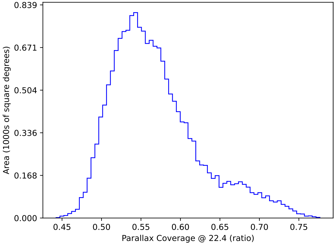
too_elab_r128_d2_griz_v3.4_10yrs WFD: Parallax Coverage @ 22.4
