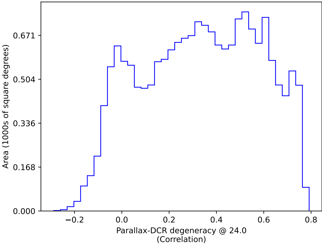
too_elab_r128_d2_griz_v3.4_10yrs WFD: Parallax-DCR degeneracy @ 24.0
