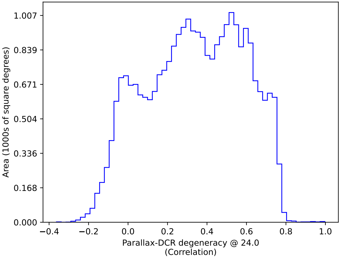
too_elab_r128_d2_griz_v3.4_10yrs All sky: Parallax-DCR degeneracy @ 24.0
