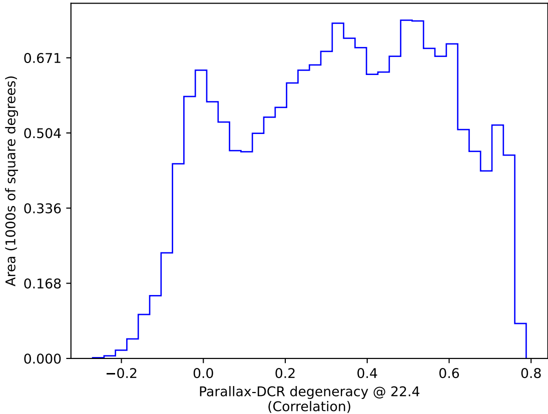
too_elab_r128_d2_griz_v3.4_10yrs WFD: Parallax-DCR degeneracy @ 22.4
