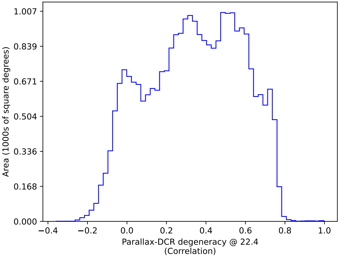
too_elab_r128_d2_griz_v3.4_10yrs All sky: Parallax-DCR degeneracy @ 22.4
