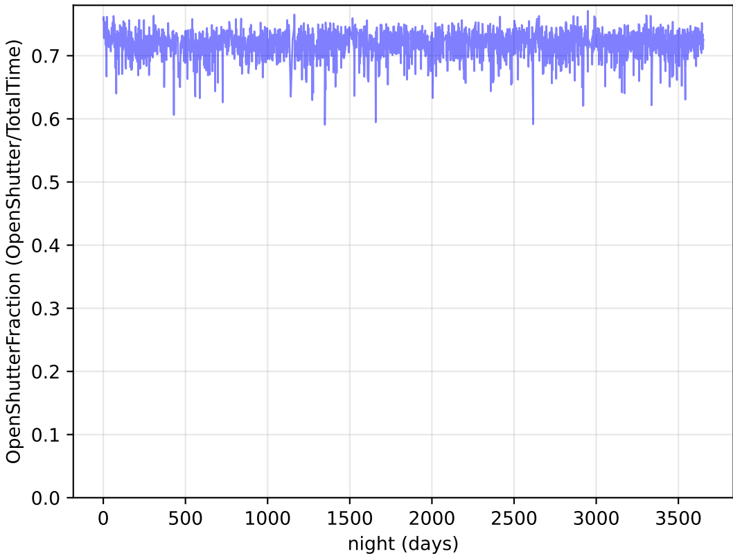
too_elab_r128_d2_griz_v3.4_10yrs Per night: OpenShutterFraction
