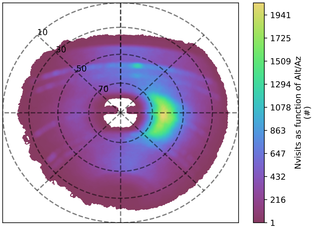
too_elab_r128_d2_griz_v3.4_10yrs y band: Nvisits as function of Alt/Az
