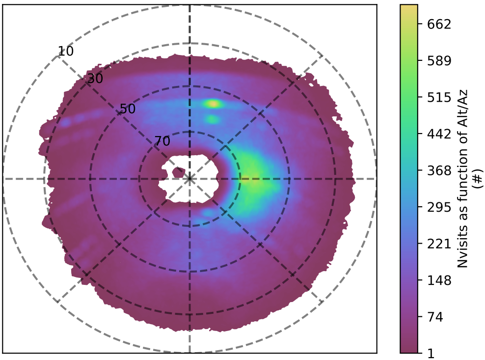
too_elab_r128_d2_griz_v3.4_10yrs u band: Nvisits as function of Alt/Az
