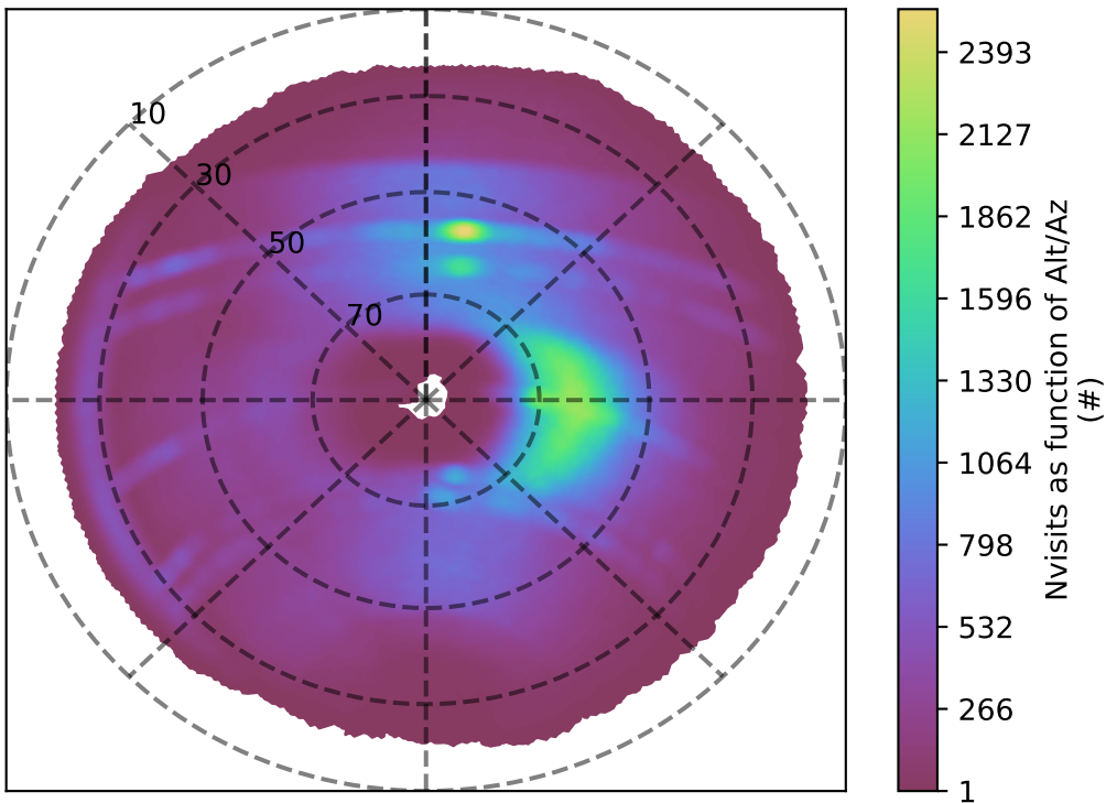
too_elab_r128_d2_griz_v3.4_10yrs r band: Nvisits as function of Alt/Az
