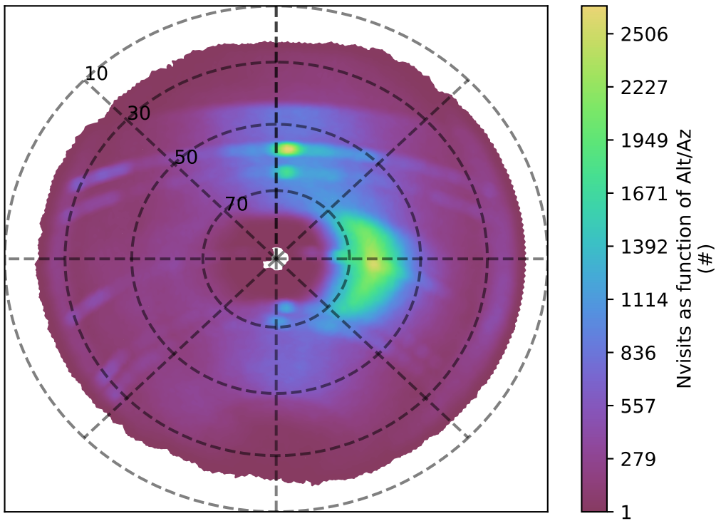
too_elab_r128_d2_griz_v3.4_10yrs i band: Nvisits as function of Alt/Az
