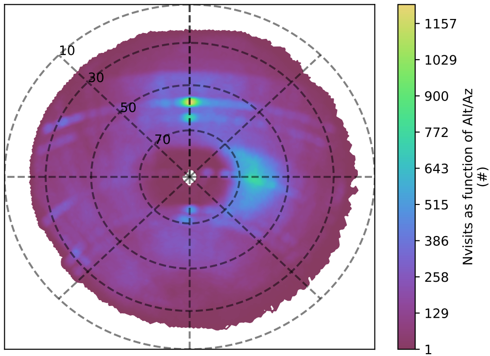
too_elab_r128_d2_griz_v3.4_10yrs g band: Nvisits as function of Alt/Az
