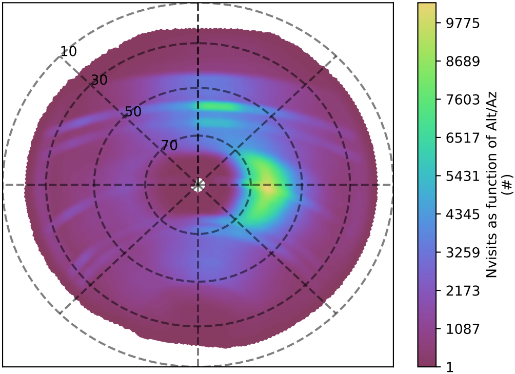
too_elab_r128_d2_griz_v3.4_10yrs all bands: Nvisits as function of Alt/Az
