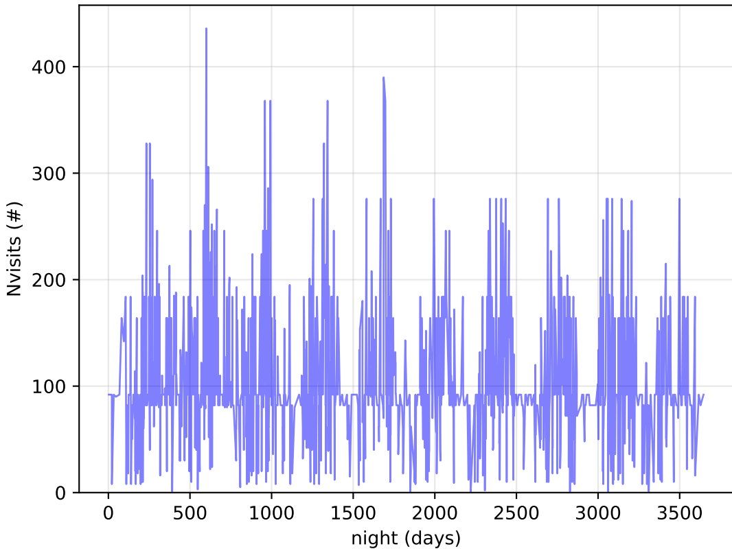
too_elab_r128_d2_griz_v3.4_10yrs DDF: Nvisits
