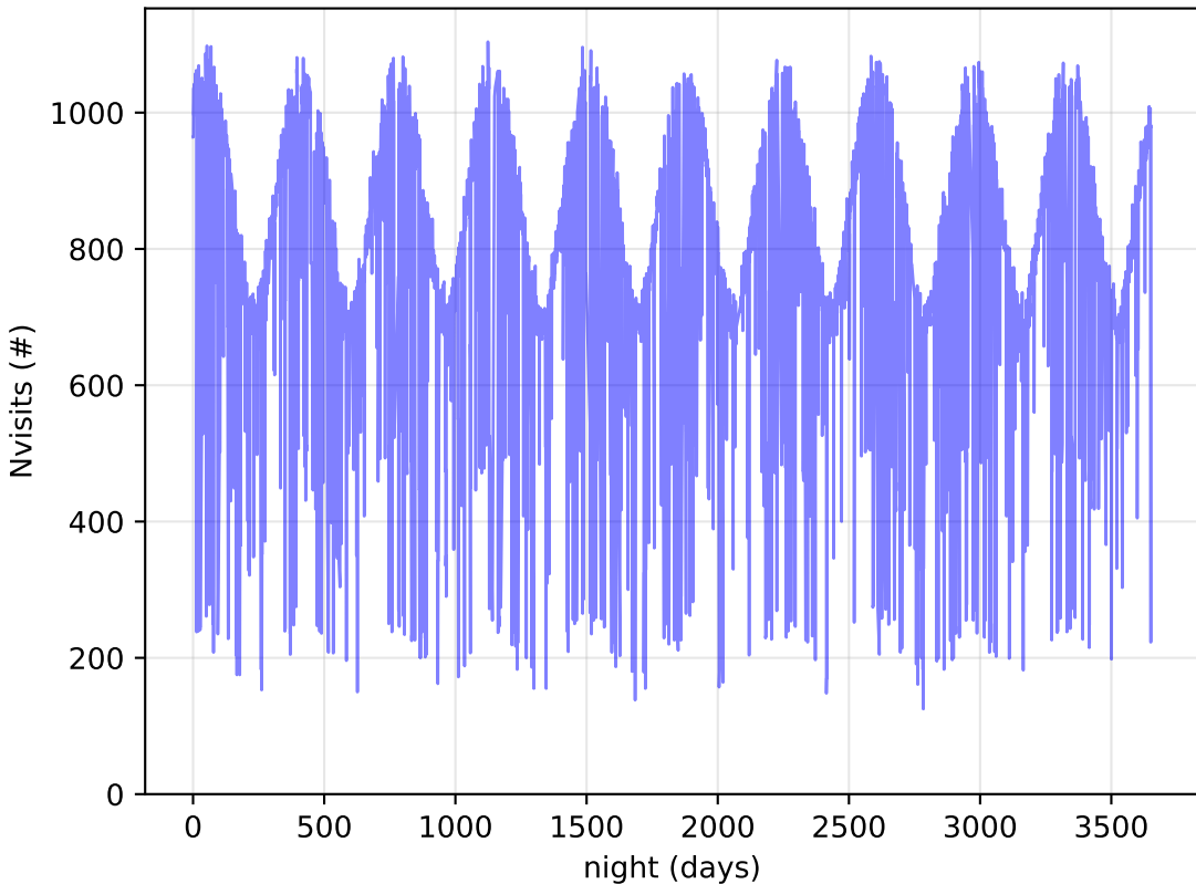
too_elab_r128_d2_griz_v3.4_10yrs All visits: Nvisits
