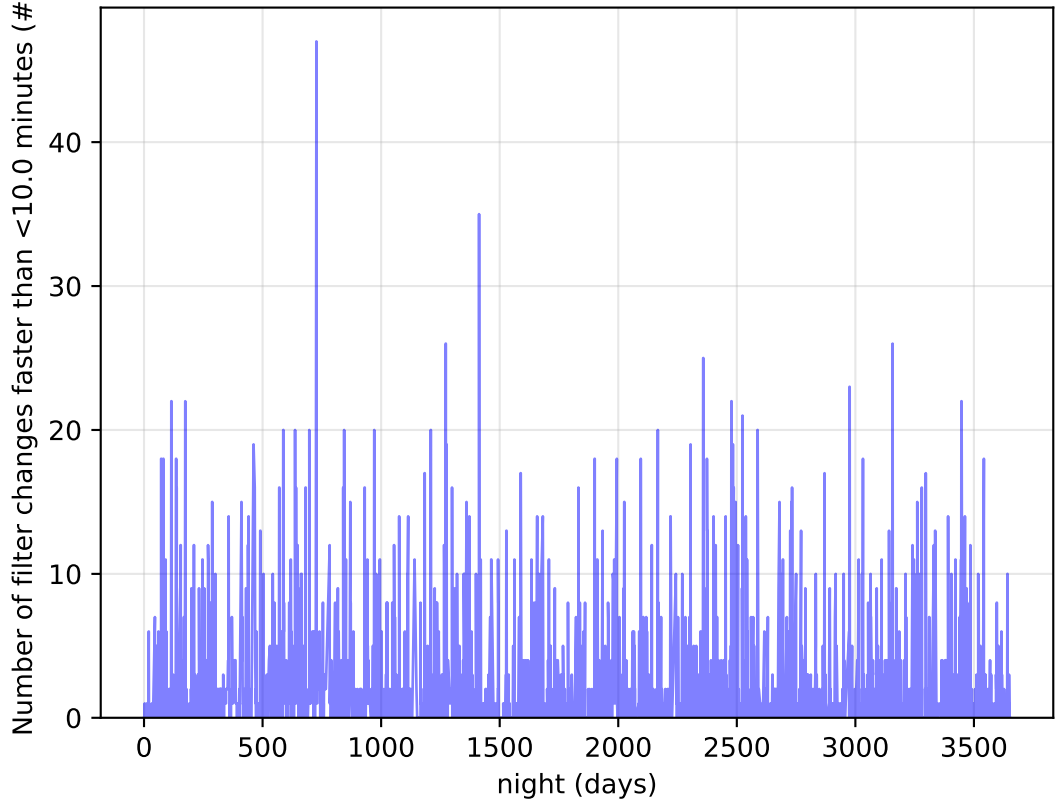
too_elab_r128_d2_griz_v3.4_10yrs Per Night: Number of filter changes faster than <10.0 minutes
